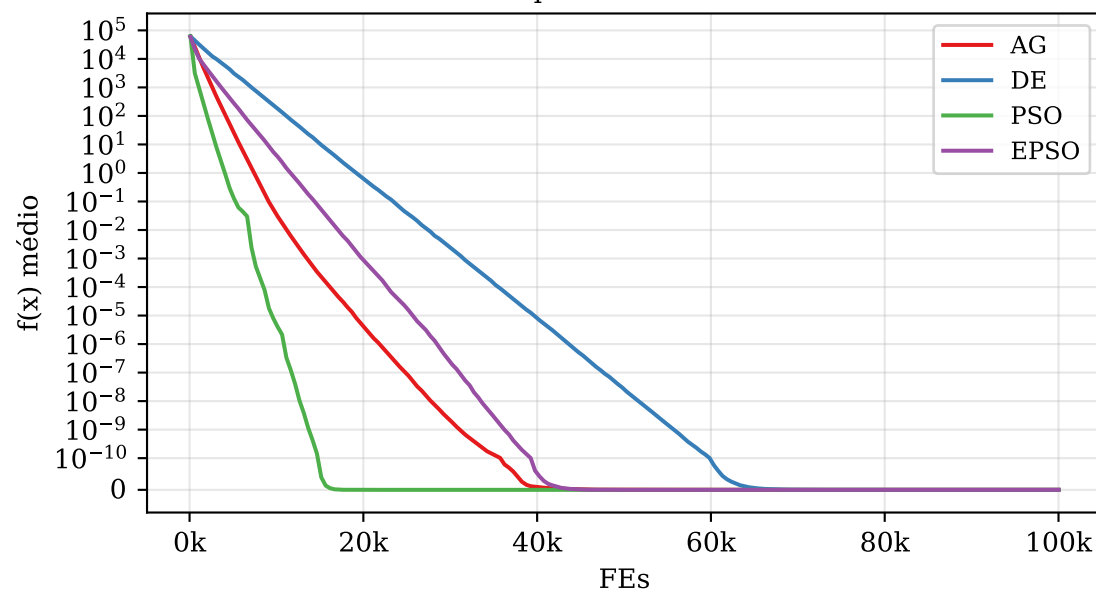
Rosenbrock — D=30
