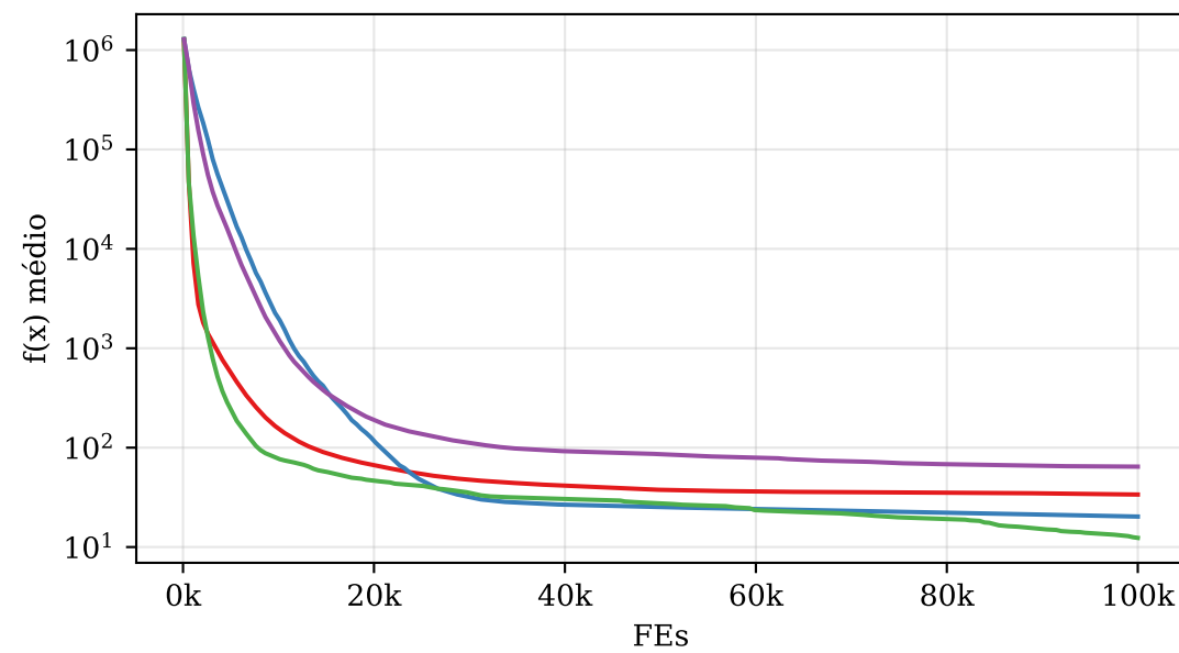
Rastrigin — D=30
